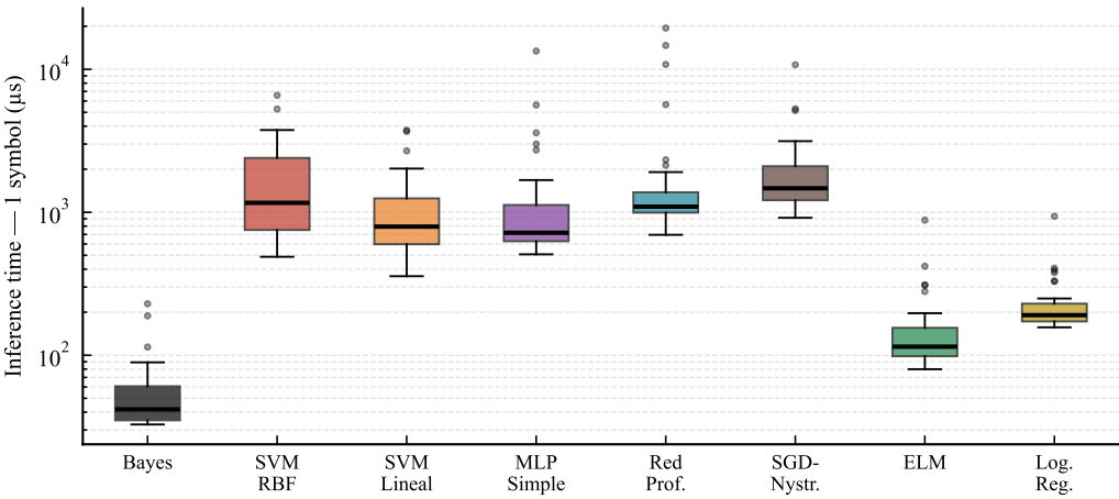
t_{inf} distribution — E_b/N_0 \in [6, 8, 10, 12] dB
